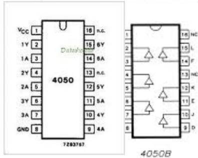
4050 : Buffer & TTL Driver (Non-Inverting)
